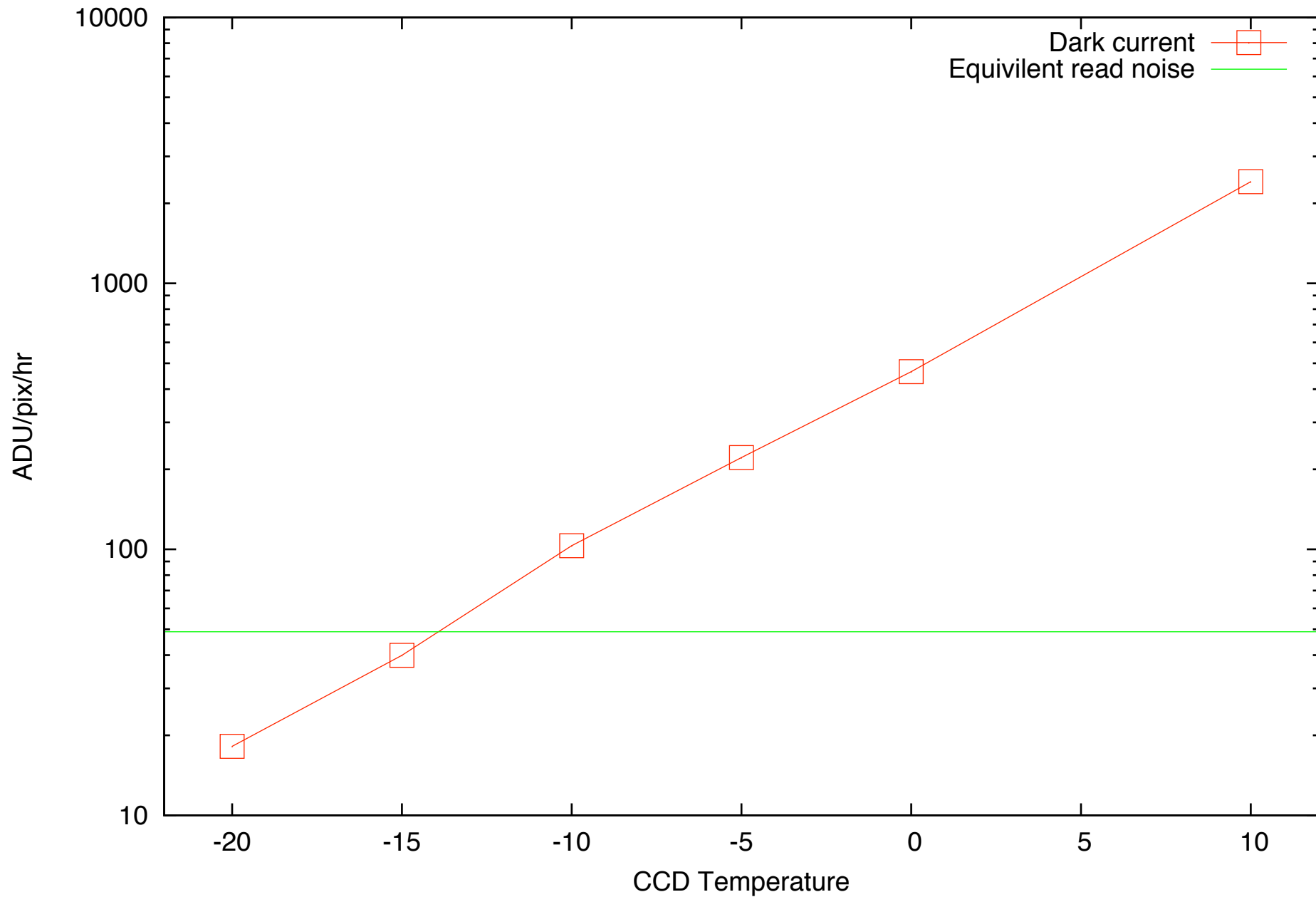
Dark Current vs CCD Temp for ST8 (2x2 binning)
